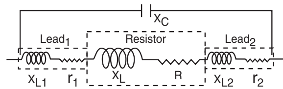
FIGURE 9. THE EQUIVALENT CIRCUIT OF A RESISTOR
