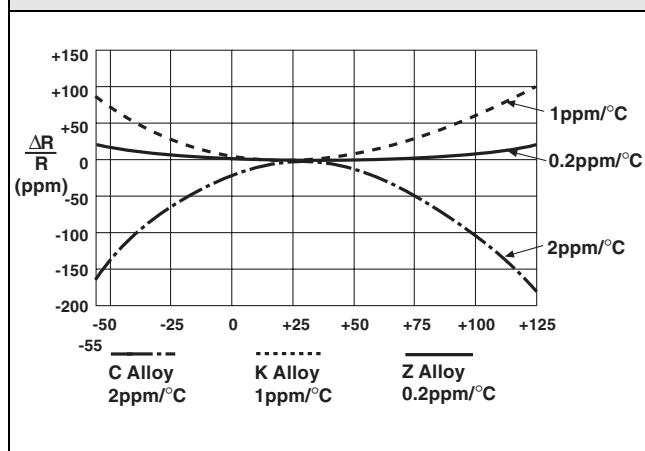
FIGURE 1. FOIL RESISTOR TCR COMPARISON OF FOIL ALLOYS IN MILITARY RANGE
