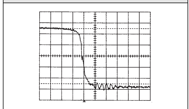
FIGURE 16. SIGNAL WITH A “NOISE-FREE” RESISTOR
