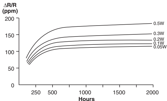
FIGURE 5. \Delta R/R = F (TIME), LOADS 0.05 TO 0.5 W, +125 °C AMBIENT
