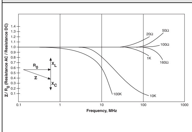
FIGURE 13. EFFECT OF OPERATION AT FREQUENCY
