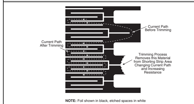
FIGURE 3. TRIMMING TO VALUES (CONCEPTUAL ILLUSTRATION)
