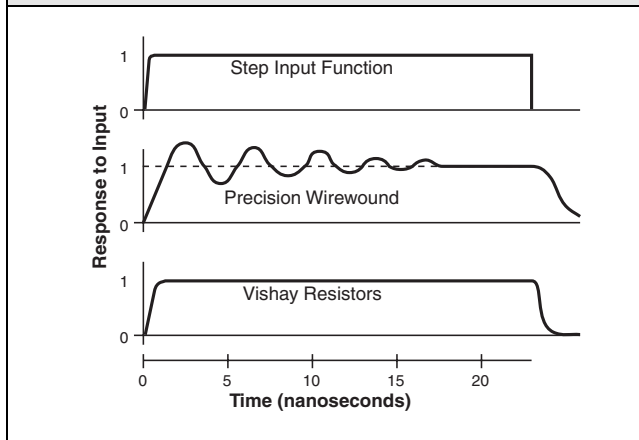
FIGURE 12. COMPARISON OF A RESPONSE TO A PULSE
