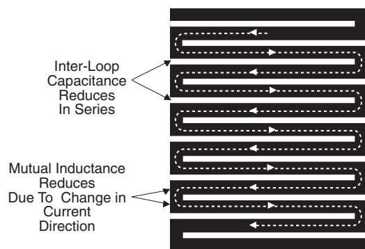
FIGURE 11. BULK METAL® FOIL PLANAR DESIGN
