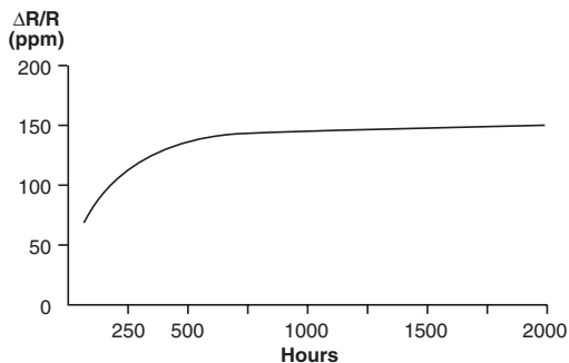
FIGURE 5. \Delta R/R = F (TIME), LOADS 0.05 TO 0.5 W, +125 °C AMBIENT
