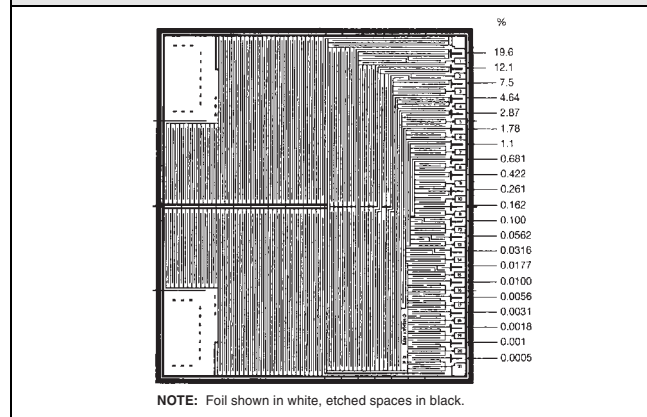
FIGURE 2. VISHAY S102C RESISTOR ELEMENT
